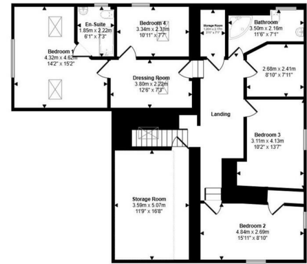
First Floor Approx 127 sq m / 1365 sq ft Denotes head height below 1.5m
